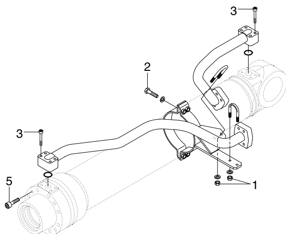
BOOM CYLINDER
