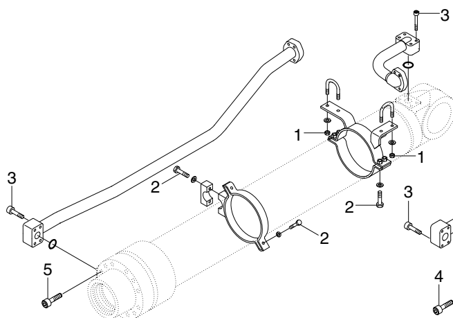
ARM CYLINDER
