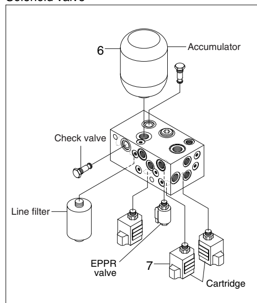
Solenoid valve
