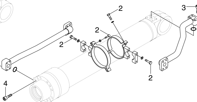
BUCKET CYLINDER
